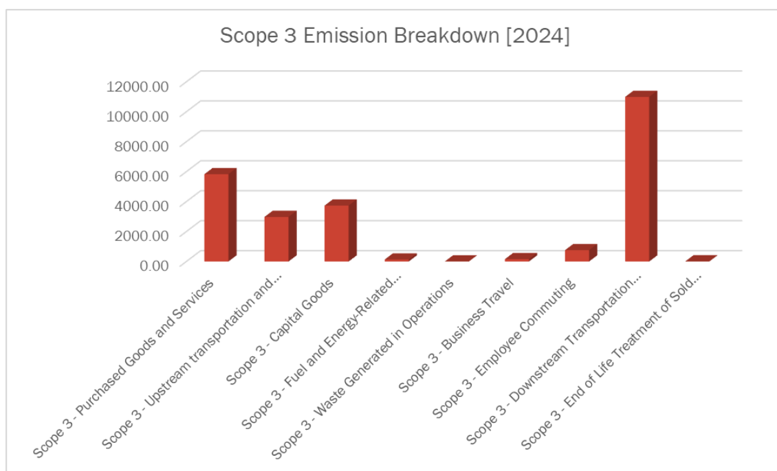
Figure 2: Scope 3 Breakdown (tonnes CO 2 equivalent)
